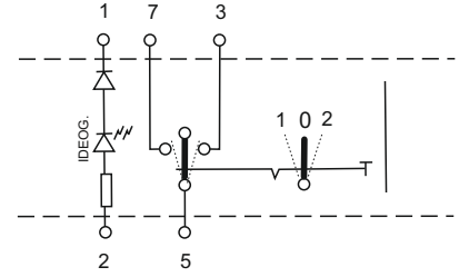
Electrical scheme V2p
