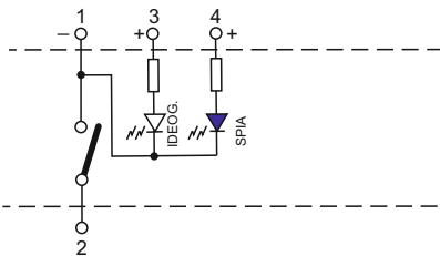
Electrical scheme D
