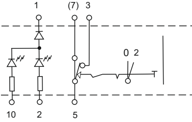
Electrical scheme M1p
