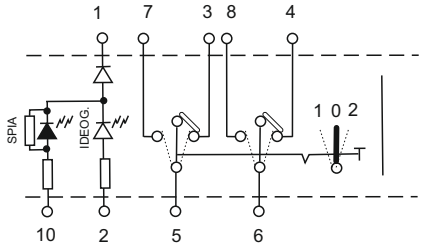
Electrical scheme L1p
