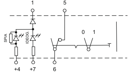
Electrical scheme F
