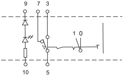
Electrical scheme G1p
